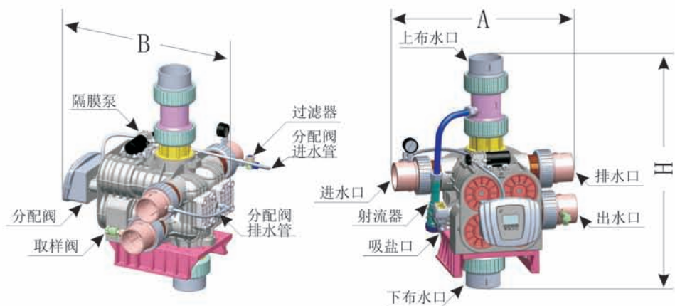
51240B(F112BS)结构图:
